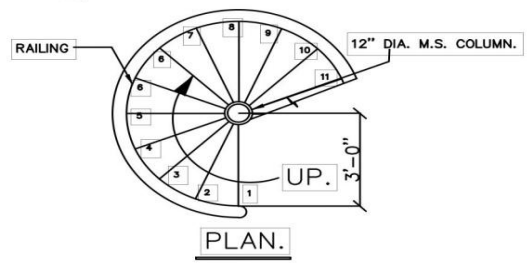
TYPICAL CAST/WROUGHT IRON SPIRAL STAIR DETAIL.
