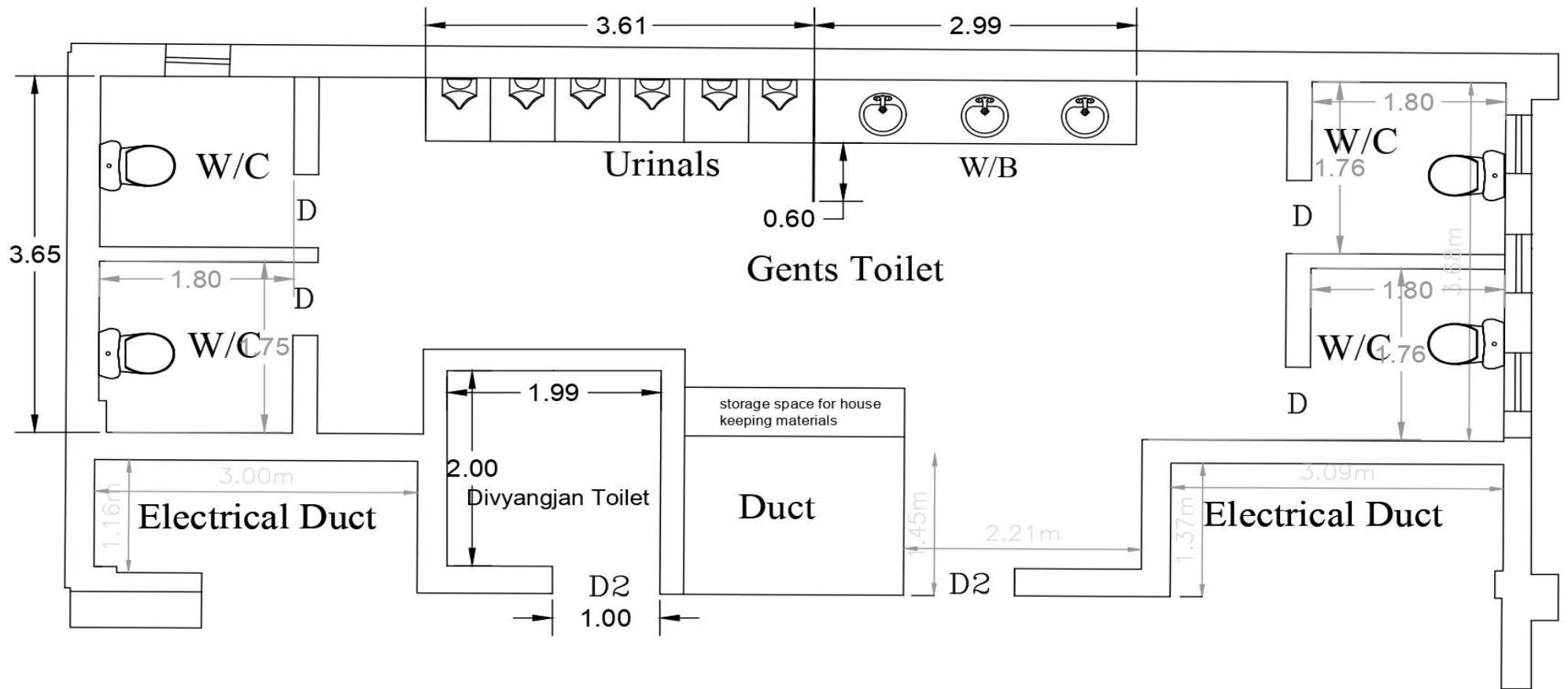
PROPOSED DIVYANGJAN TOILET PLAN AT MAIN LAB BUILDING CREST CAMPUS, HOSAKOTE.
