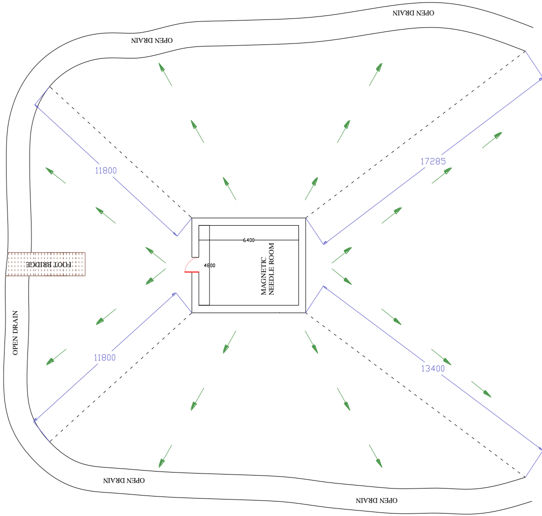
MAGNETOSPHERE DOME BUILDING PLAN AT 6.0M LEVEL
