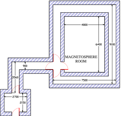
PLAN AT 0.50M LEVEL
