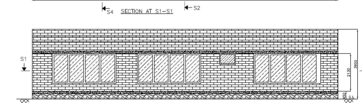
FRONT ELEVATION (VIEW FROM SOUTH)
