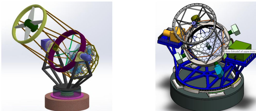
Figure 1 Conceptual design of 1.3m Prototype Segmented Mirror Telescope (left) and 10m class National Large Optical Telescope (right).
